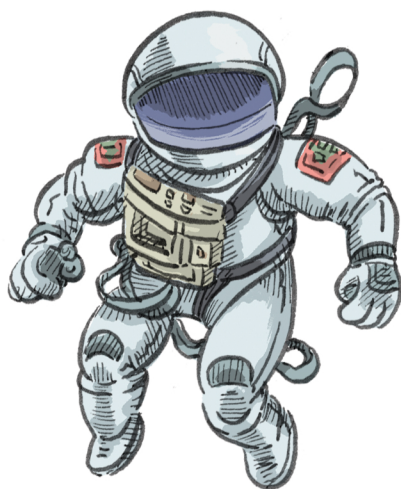
Astronaut
